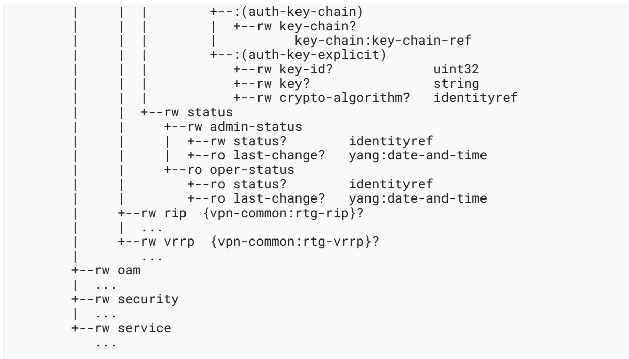
Figure 15: IS-IS Routing Tree Structure
