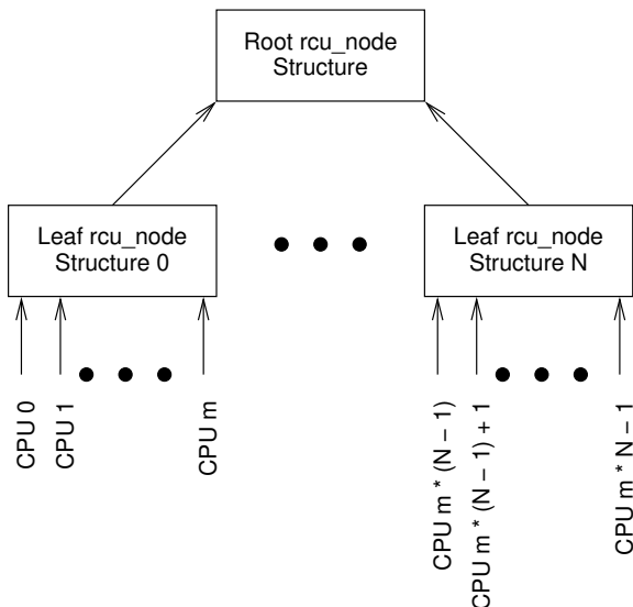
Figure 7.9: Locking Hierarchy
