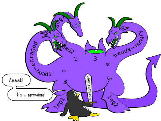
Figure 10.14: Partitioning Problems
