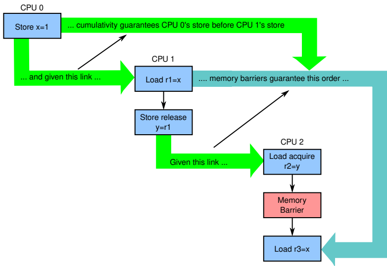
Figure 15.9: Cumulativity
