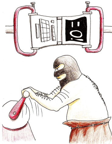
Figure 11.2: Rationalizing Validation
