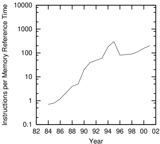
Figure 17.6: Instructions per Local Memory Reference for Sequential Computers
