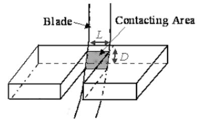
Figure 7.9: Saw Kerf
